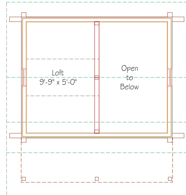
Second Floor 50 sq-ft
