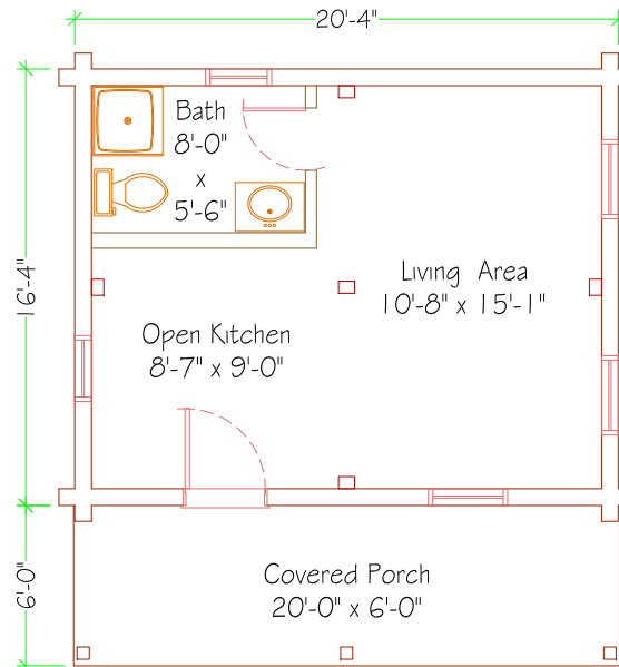
First Floor 330 sq-ft
