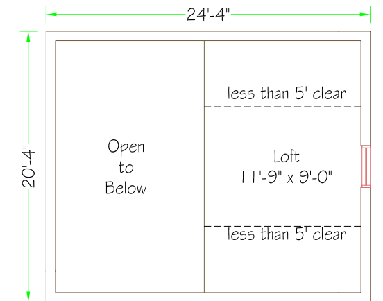
Second Floor Plan 110 sq-ft
