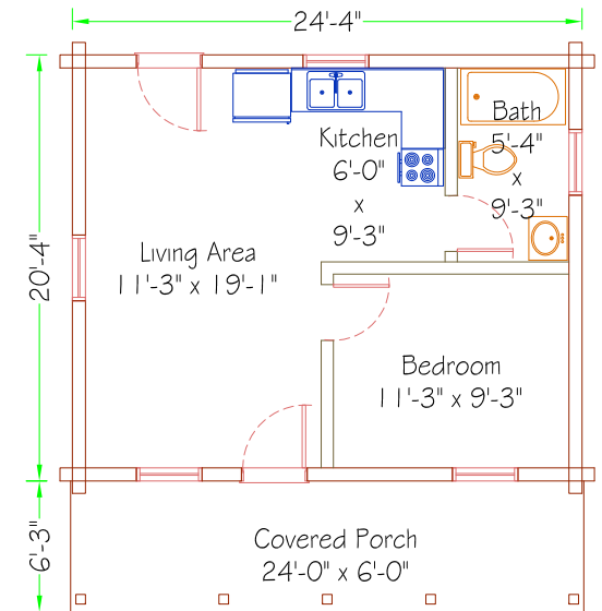
First Floor Plan 490 sq-ft
