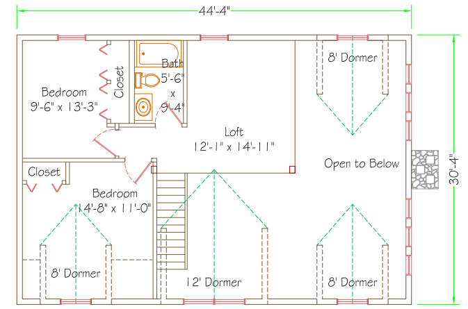
Second Floor 675 sq-ft
